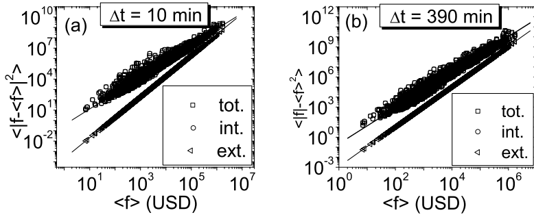
Fig. 1 – Scaling of q = 2 central moments of activities and fitted linear trends. (a) \Delta t = 10 minutes. \alpha(2; \text{tot}) \approx \alpha(2; \text{int}) = 0.773 \pm 0.003 . (b) \Delta t = 390 minutes = 1 trading day. \alpha(2; \text{tot}) \approx \alpha(2; \text{int}) = 0.885 \pm 0.005 . Errors are estimated from the linear fit on the log-log plot. Note that, although the errors are very low due to the large number of data points, there is pronounced unexplained variance around the expected scaling of total and internal noise. This can be reduced significantly if one takes the system structure (in our case the clustering of stocks into market sectors) into account [9].
