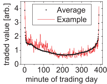
Fig. 3 – The intraday pattern of trading activity, which is calculated as the average of the individual daily time series. The activity during one example day is given for comparison.
