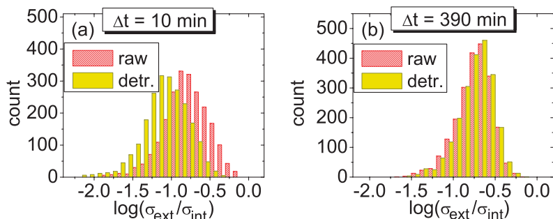
Fig. 5 – Histogram of the ratios of the internal and external standard deviations for all stocks, both for raw and detrended time series. The comparison shows that external influence is stronger on a daily time scale than for fine resolution data. (a) \Delta t = 10 minutes. Detrending with the intraday pattern removes the spurious external driving force due to daily peaks in activity. This decreases the measured external contribution in fluctuations. (b) \Delta t = 390 minutes = 1 trading day. Detrending does not change behavior measured on a daily (or longer) scale.
