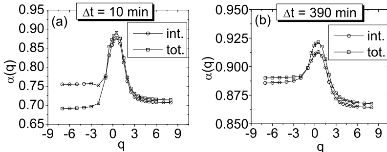
Fig. 2 – The \alpha(q) multiscaling exponents for all three types of activity. \alpha(q; \text{ext}) \equiv 1 . (a) \Delta t = 10 minutes. (b) \Delta t = 390 minutes = 1 trading day.
