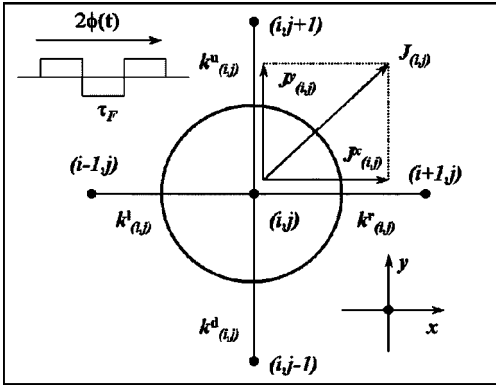
FIG. 1. Schematic diagram illustrating the parameters of the studied two-dimensional driven diffusion problem. A particle on the site (i, j) hops to its neighboring sites with hopping rates k_{i,j}^{\gamma} , defined by both the potential barriers between these sites and by the alternating field. The time-dependent behavior of the external field is shown on the top left.
