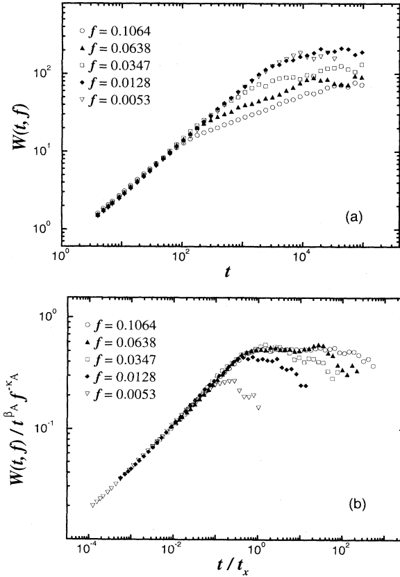
FIG. 11. DPD universality class. (a) Plot of the global width W as a function of time t and the moving phase interface. The system size is L = 10480 and each result was averaged over 50 realizations of the disorder. (b) Data collapse of the widths according to (5.11).
