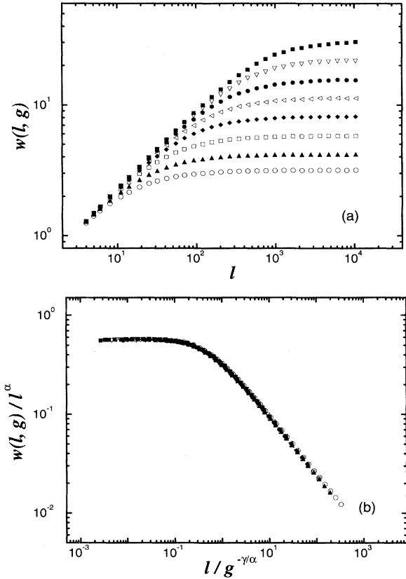
FIG. 15. Simulation results for the width w(\ell, g) of the pinned interface in 1 + 1 dimensions, where g is the gradient in \rho . (a) The widths for values of the gradient ranging from 1/70 to 1/7680 . The system size is 10480 and each result is averaged over 30 realizations of the disorder. (b) Data collapse of these results according to the scaling form (B4), using the values of the exponents given in (B5).
