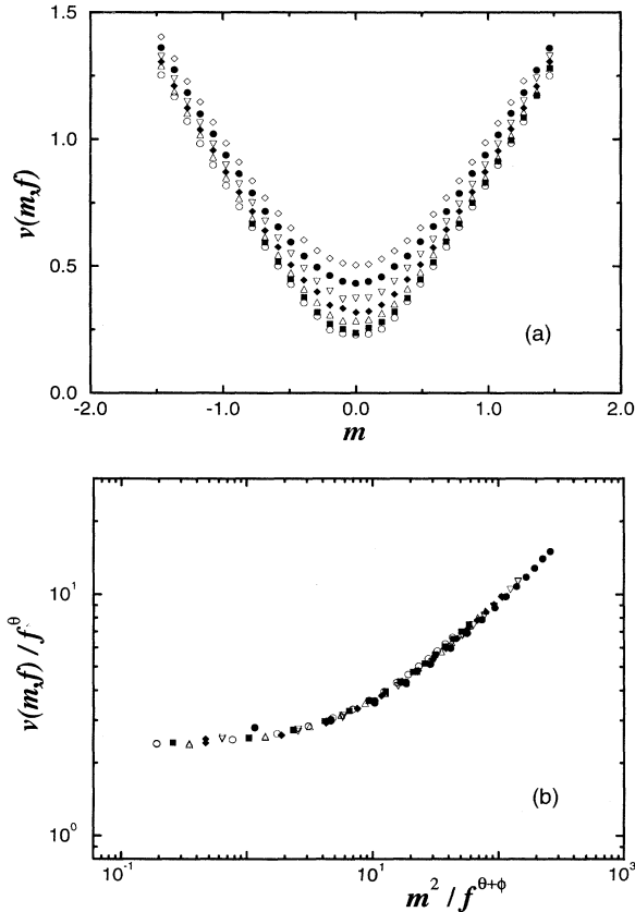
FIG. 5. DPD-2 model. (a) Dependence on the tilt m of the average velocity in 1 + 1 dimensions. Data for different forces f are indicated by different symbols, ranging from 0.0149 (bottom curve) to 0.0719 (top curve). The system size is L = 512 and each result was averaged over 30 realizations of the disorder. (b) Data collapse of the velocities according to (4.7) using the values for the DPD-2 model exponents (Table I).
