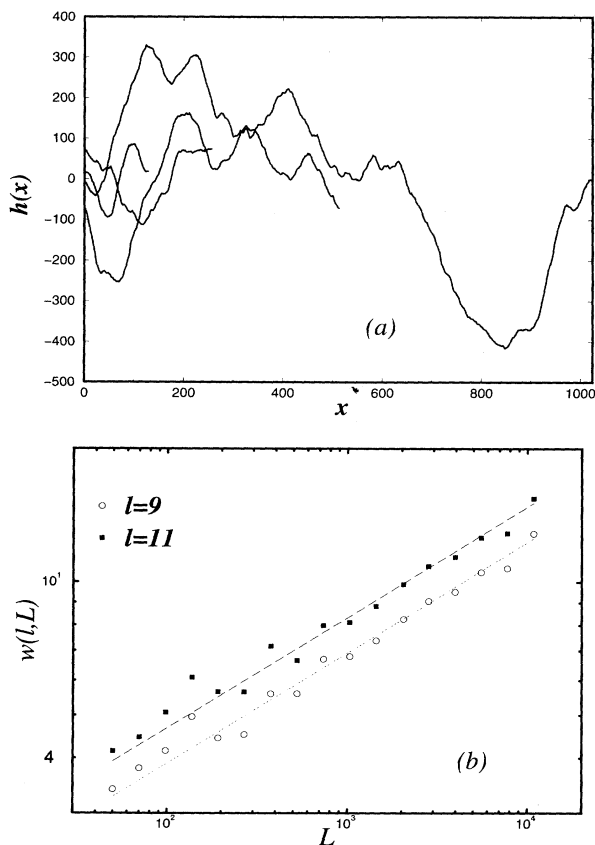
FIG. 12. Anomalous scaling of the local width for the QEW universality class. (a) Interfaces generated with the QEW-2 model, at the depinning transition, for system of sizes L = 128, 256, 512, 1024 . We note that the local slopes increase with the system size. (b) Plot of the scaling of the local width as a function of L , for two given values of \ell . The fit corresponds to \alpha_G - \alpha_P \approx 0.25 .
