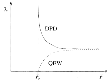
FIG. 9. Schematic representation of the scaling behavior of the coefficient \lambda of the nonlinear term for the two universality classes. For the DPD universality class we see that \lambda diverges at the depinning transition, while for the QEW universality class it vanishes to zero at the transition.
