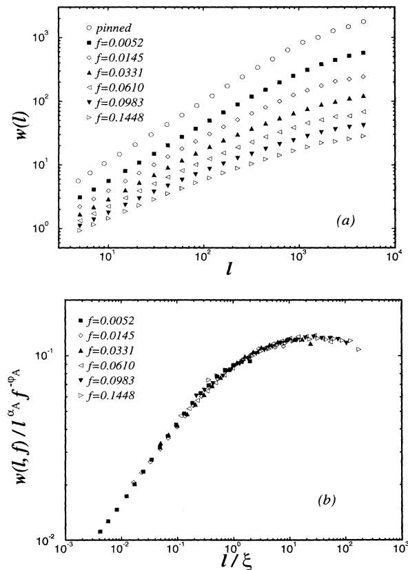
FIG. 13. QEW universality class. (a) Plot of the local width in the moving phase for several values of the reduced force. The system size is L = 5524 and each result was averaged over 100 realizations of the disorder. (b) Data collapse of the widths according to (5.3).
