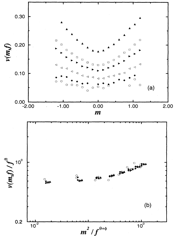
FIG. 8. RFIM. (a) Dependence on the tilt m of the average velocity in 2 + 1 dimensions. Data for different values of the force f are indicated by different symbols, ranging from 0.014 (bottom curve) to 0.143 (top curve). The system size is L^2 = 40 \times 40 and \Delta = 3 (SA regime). (b) Data collapse of the velocities according to (4.7) using the values for the RFIM exponents (Table I).
