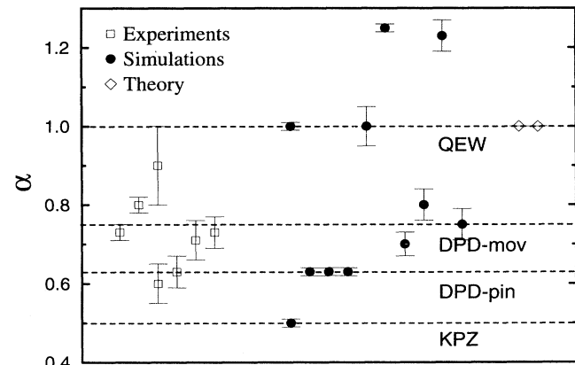
FIG. 2. Values of the roughness exponent \alpha from most of the experiments, simulations, and theoretical works reported in the literature. The experimental points are, reading from left to right, from Refs. [8–10] (a range of values is reported of which the extremes are plotted), [12–17,11]. The simulation points are, reading from left to right, from Refs. [17] (a range of values is reported of which the extremes are plotted) and [29,12–17,32,31,34,33,40,27,28,45,46]. Finally, the theoretical points, again reading from left to right, are from Refs. [48] and [49]. Visually apparent is the wide spread of the results. To guide the eye, we indicate the values of \alpha predicted by the KPZ equation with annealed disorder (bottom line), the DPD universality class in the pinned phase and moving phases (middle lines), and the QEW universality class (top line). We can see that most results for simulations and theoretical calculations are close to either the DPD or the QEW line. However, for the experimental results, the agreement is not so good. In the text we argue that the reasons for these disagreements are the crossover present in the moving phase for both universality classes and the fact that for the DPD universality class \alpha_M \neq \alpha_P .
