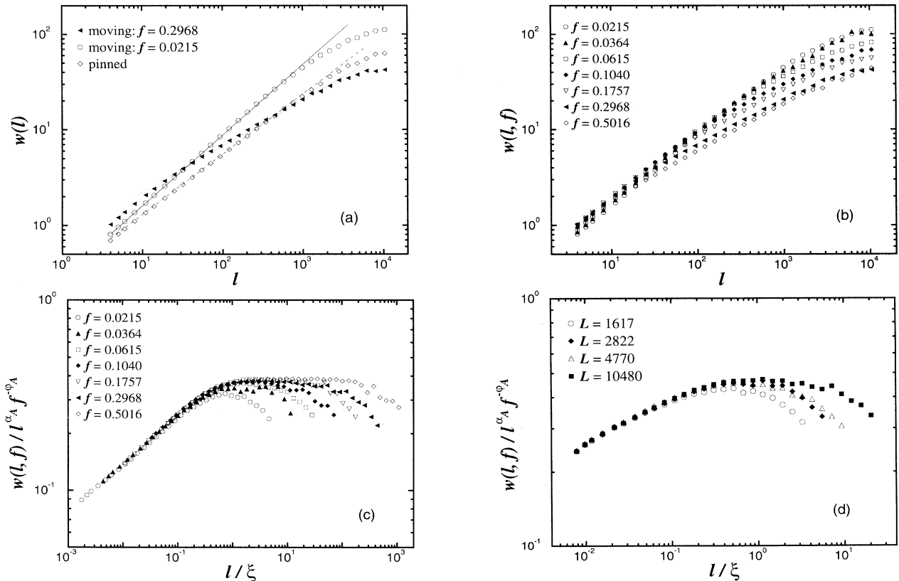
FIG. 10. DPD universality class. (a) Plot of the local width w as a function of l for a pinned and a moving interface. The different roughness exponent is clear. The system size is L = 10480 and each result was averaged over 50 realizations of the disorder. (b) Plot of the local width in the moving phase for several values of the driving force. (c) Data collapse of the widths according to (5.3). (d) Data collapse for f = 0.0583 and for systems of different size L . Visually apparent is the fact that the deviations from scaling observed in (c) are due to finite size effects.
