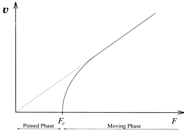
FIG. 1. Depinning transition. In the “pinned phase” F < F_c , the velocity of the interface is zero. In the “moving phase” F > F_c , the interface moves with an average velocity v \equiv v(F) , where v(F) \sim (F - F_c)^\theta for F close to F_c and v(F) \sim F for F \gg F_c . Thus the velocity plays the role of the order parameter of the transition.
