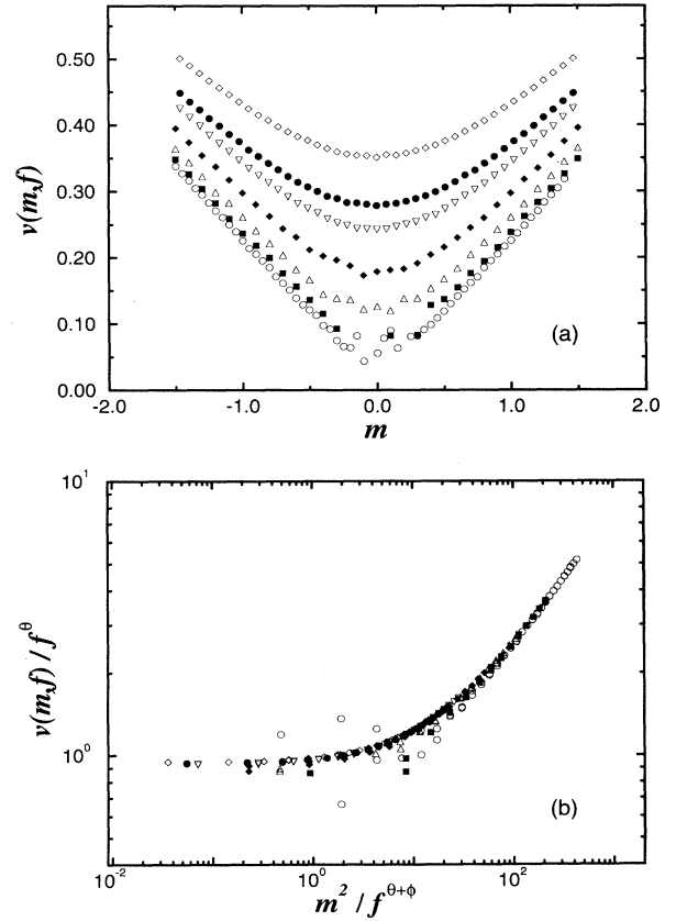
FIG. 6. DPD-3 model. (a) Dependence on the tilt m of the average velocity in 1 + 1 dimensions. Data for different values of the force f are indicated by different symbols, ranging from 0.0204 (bottom curve) to 0.2454 (top curve). The system size is L = 1024 and each result was averaged over 30 realizations of the disorder. (b) Data collapse of the velocities according to (4.7) using the values for the DPD-3 model exponents (Table I).
