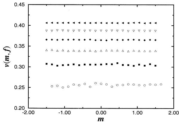
FIG. 7. QEW-1 model. Dependence on the tilt m of the average velocity in 1 + 1 dimensions. Data for different values of the force f are indicated by different symbols, ranging from 0.0125 (bottom curve) to 0.075 (top curve). The system size is L = 1024 and each result was averaged over 30 realizations of the disorder. We can see clearly that \lambda = 0 .
