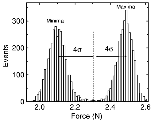
FIG. 4. Distribution of maxima and minima in the periodic regime. ( d_c=16 mm, d_g=0.9 mm and H=60 mm.) The large separation between the peaks of the histograms for the maxima and minima characterizes the periodic regime.
