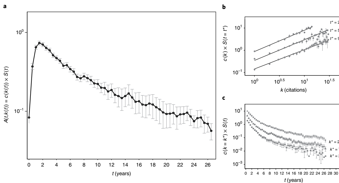
Fig. 1 | Universal patterns in the decay of human collective memory. a , Average number of citations received each semester by papers published in Physical Review B ( A(t) ). b , Average number of citations received by a paper as a function of the cumulative citations received by that paper ( \alpha c(k) ). Different curves represent different ages. c , Average number of citations received by papers with the same number of cumulative citations as a function of their age ( \alpha S(t) ). Different curves represent groups of papers with a different number of total citations. Error bars represent standard errors.
